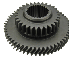
AGW 750701 COUNTER SHAFT MAIN GEAR TEETH : 30/56 81804754,C5NN7113D 91NH7113AA FORD 2000,3000,3600,3610 4000
